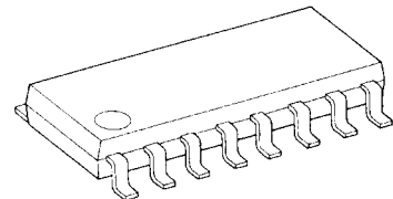
SOP16-P-225-1.27
